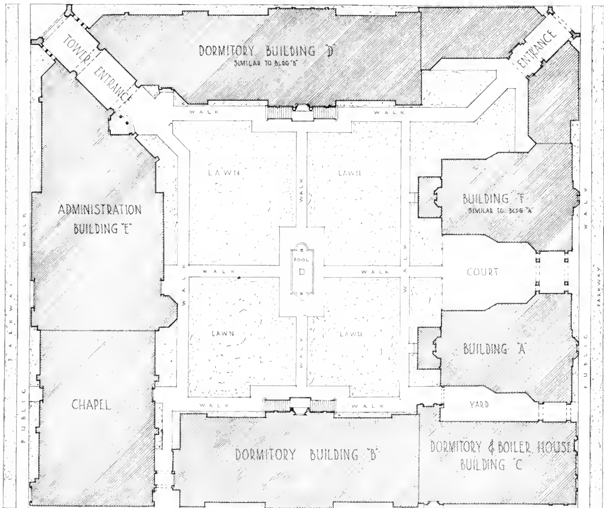
PLOT PLAN
